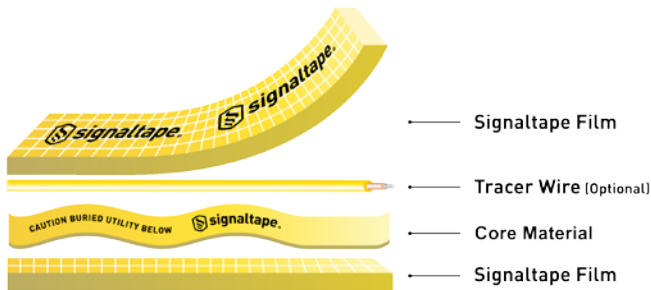
Figure 2 - Signaltape Construction
