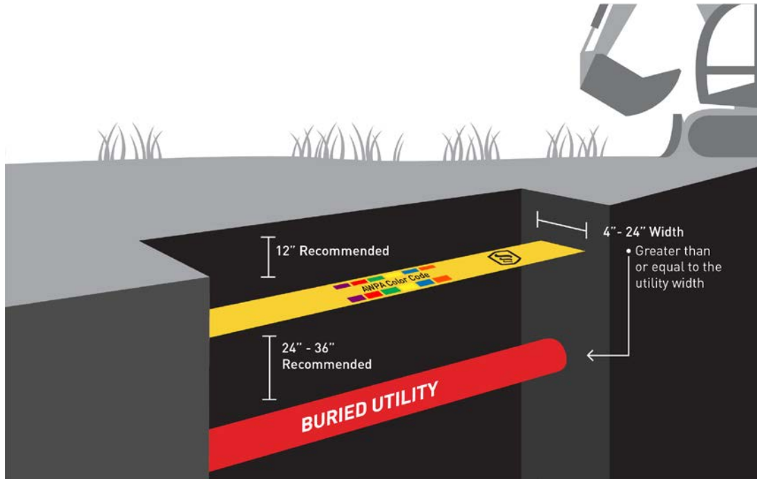
Figure 1 - Signaltape Installation
